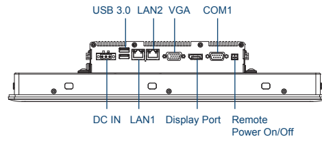
Rear I/O
